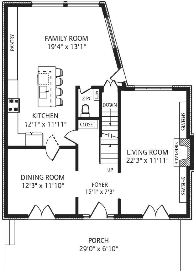
MAIN FLOOR 1,135 SQUARE FEET
