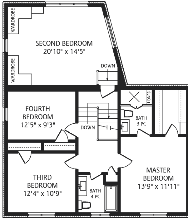
SECOND FLOOR 1,130 SQUARE FEET ALL MEASUREMENTS SHOULD BE CONSIDERED APPROXIMATE 5 FOOT SCALE
