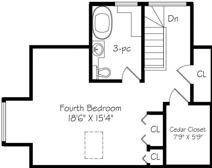
Third Floor - 491 Square Feet
