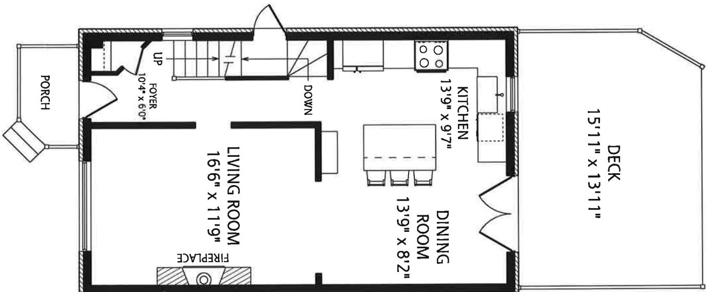
MAIN FLOOR 650 SQUARE FEET
