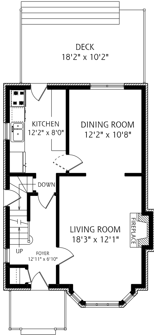
MAIN FLOOR
