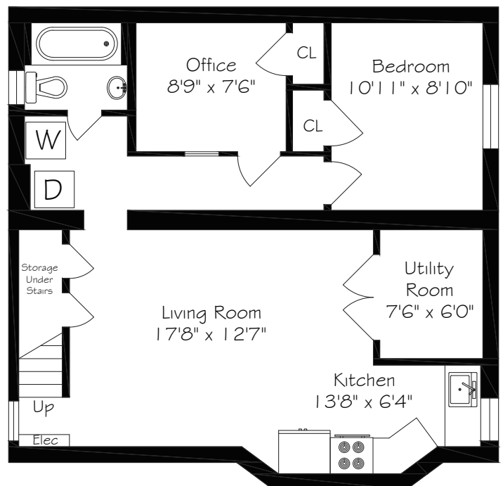
Lower Level - 857 Square Feet
