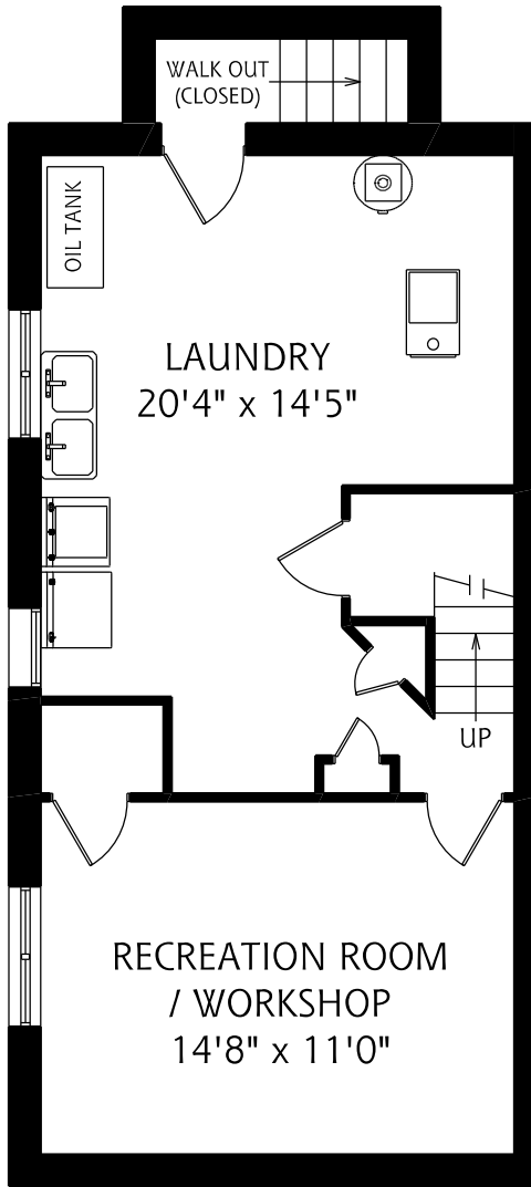
LOWER LEVEL
