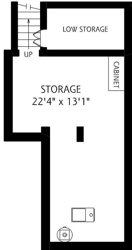
LOWER LEVEL
