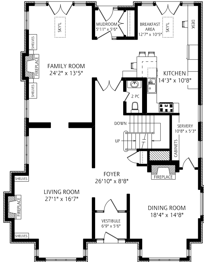
MAIN FLOOR 2,000 SQUARE FEET
