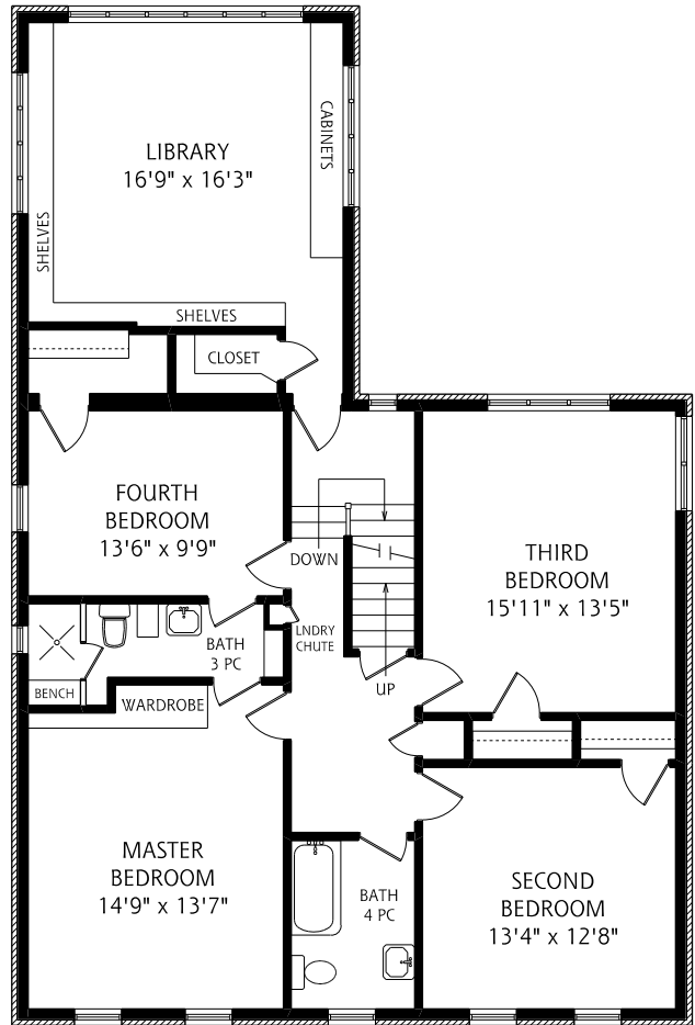
SECOND FLOOR 1,580 SQUARE FEET
