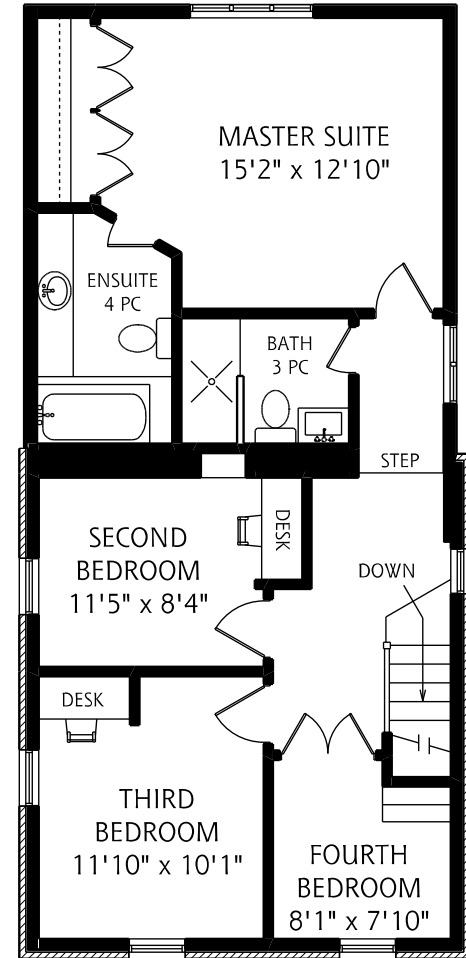
SECOND FLOOR
