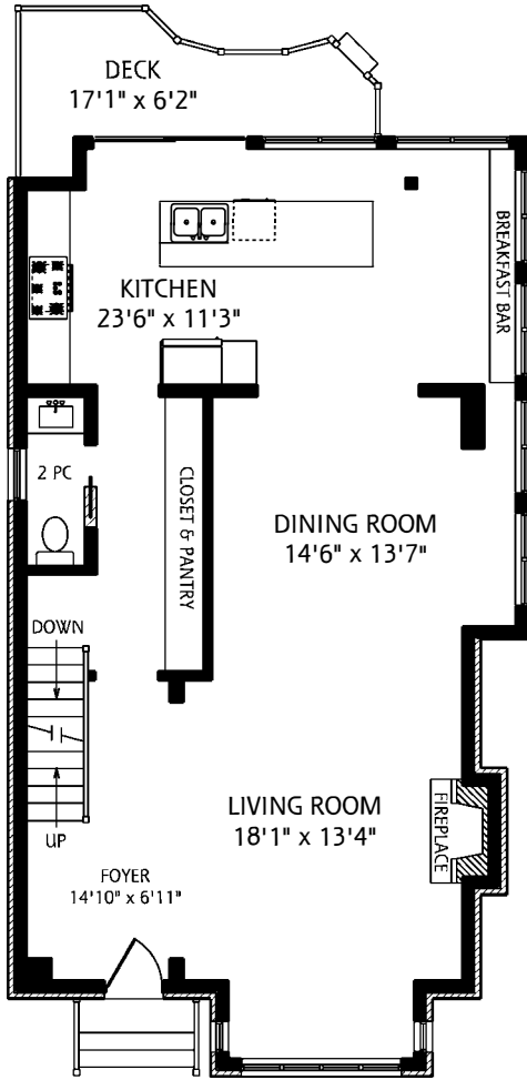
MAIN FLOOR 1,045 SQUARE FEET
