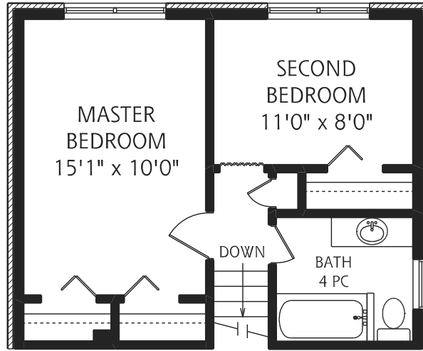
SECOND FLOOR 445 SQUARE FEET
