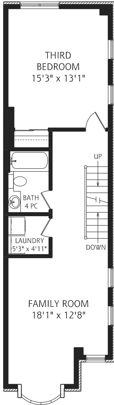
SECOND FLOOR 705 SQUARE FEET
