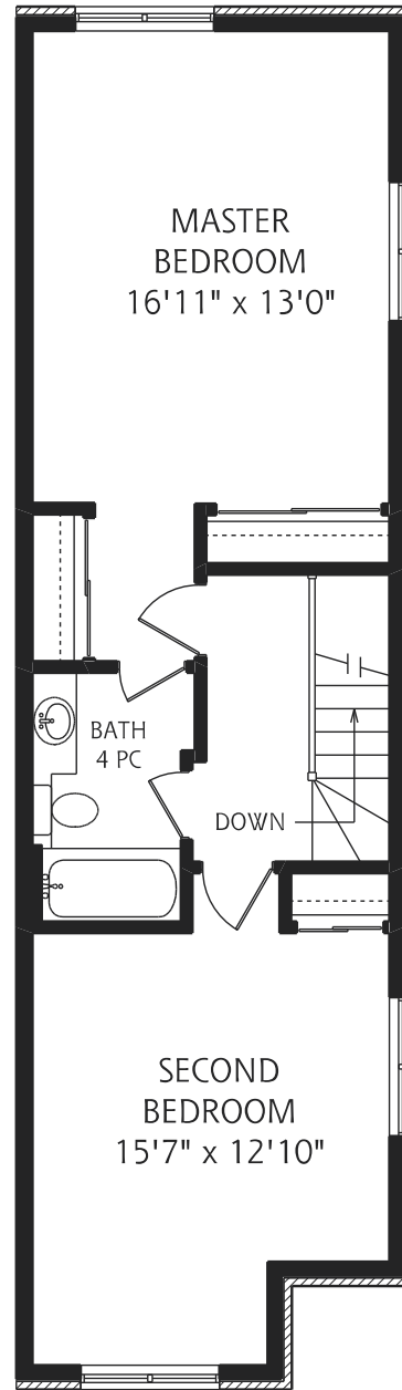
THIRD FLOOR 700 SQUARE FEET
