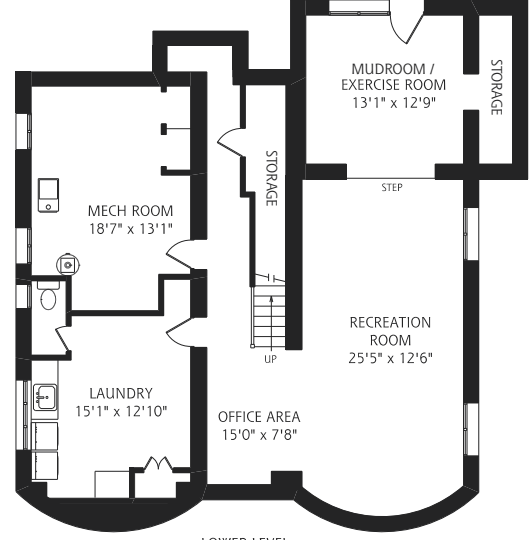
LOWER LEVEL 1,575 SQUARE FEET
