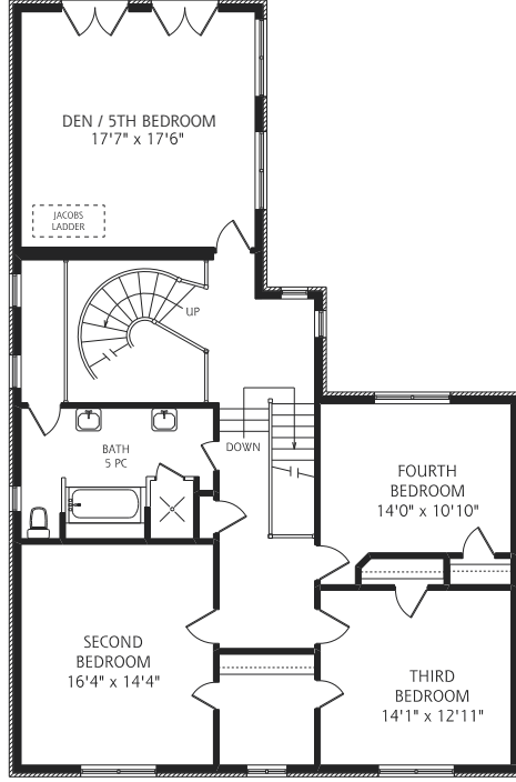
SECOND FLOOR 1,675 SQUARE FEET ALL MEASUREMENTS SHOULD BE CONSIDERED APPROXIMATE 1/5 FOOT SCALE
