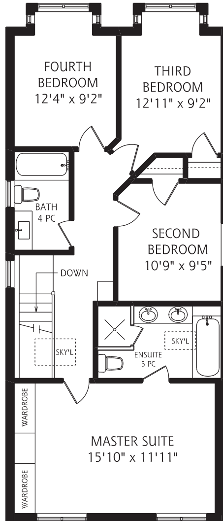
SECOND FLOOR
