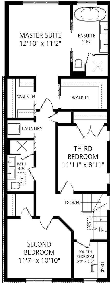
SECOND FLOOR
