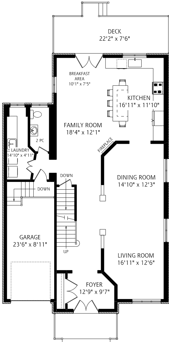
MAIN FLOOR 1,430 SQUARE FEET
