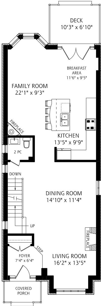
MAIN FLOOR 1,160 SQUARE FEET
