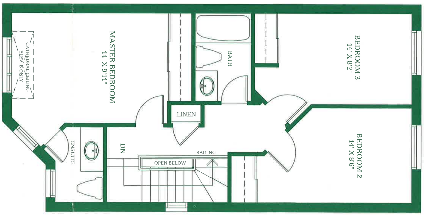
UPPER FLOOR ELEVATION B
