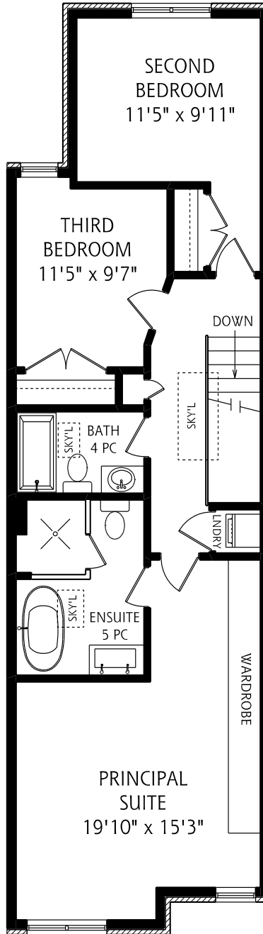
SECOND FLOOR 880 SQUARE FEET
