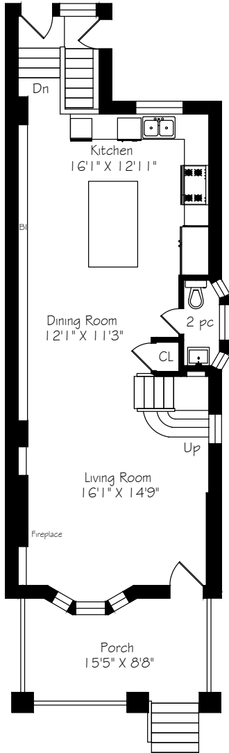
Main Floor 856 Square Feet
