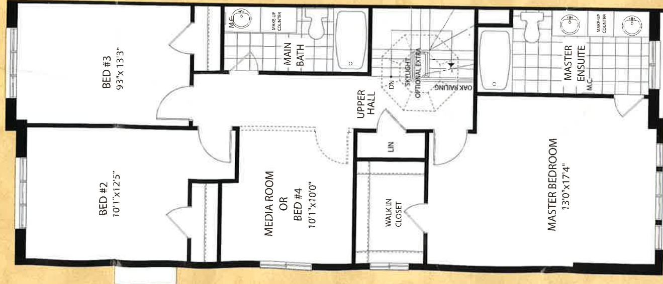
Second Floor Plan - Elevation B (4 Bedroom with Standard Master Ensuite)
