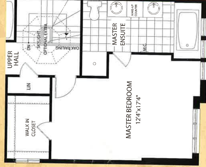
Second Floor Plan - Elevation A (4 Bedroom with Optional Extra Upgrade Master Ensuite)
