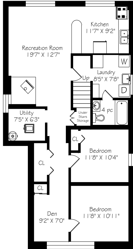
Lower Level 1182 Square Feet
