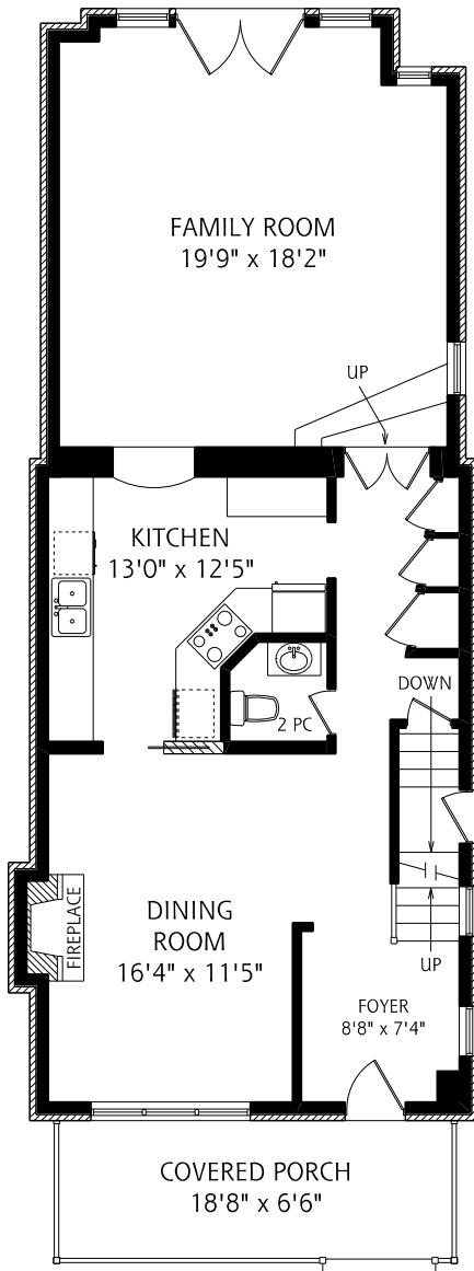
MAIN FLOOR 1,075 SQUARE FEET
