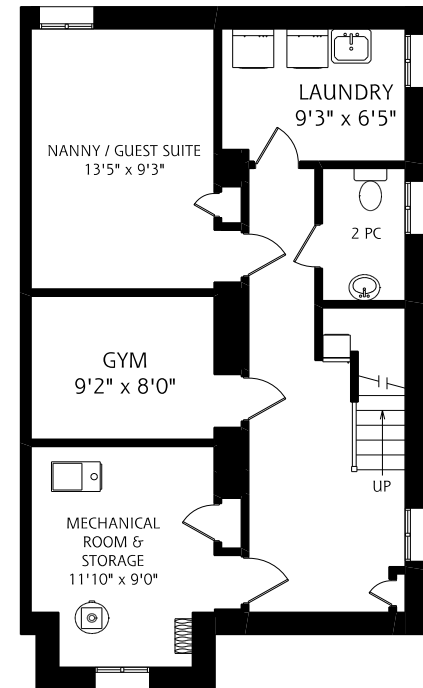
LOWER LEVEL
