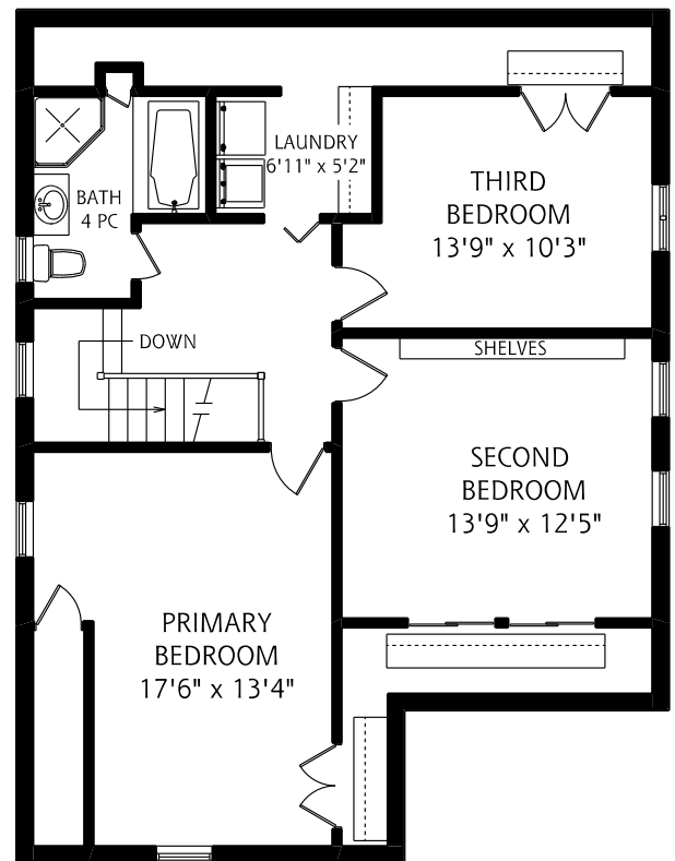
SECOND FLOOR 935 SQUARE FEET
