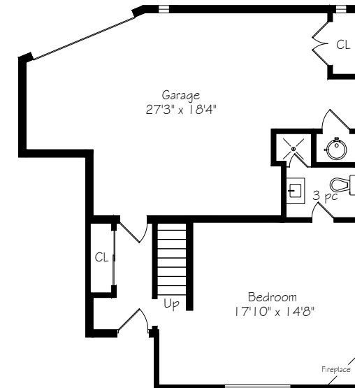
Coach House Main Floor 421 Square Feet Garage - 470 Square Feet
