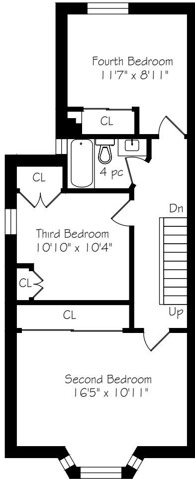
Second Floor 732 Square Feet
