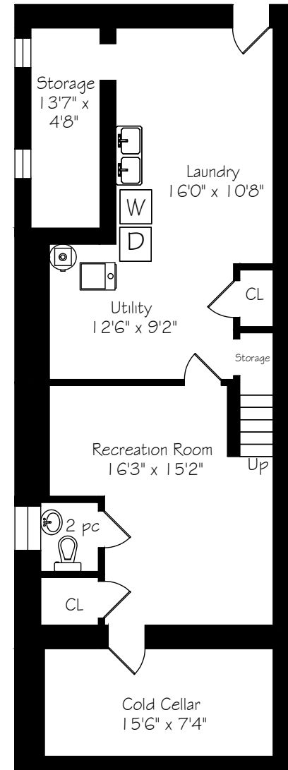
Lower Level 789 Square Feet
