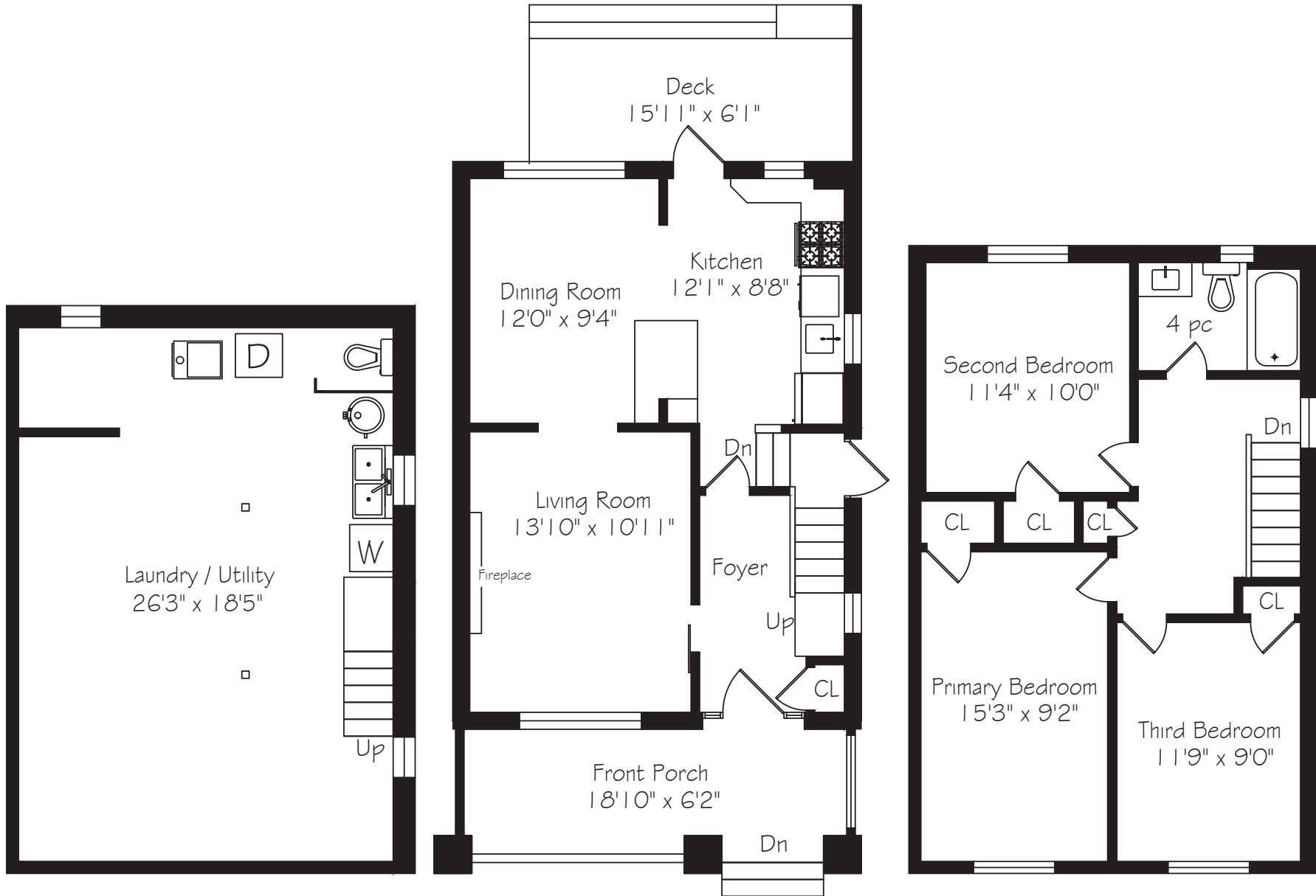
Lower Level 560 Square Feet
