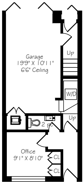
Laneway Main 286 Square Feet + 253 Garage
